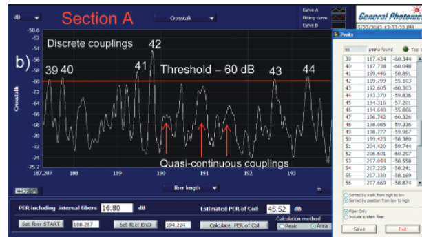
Fig. 2 a) X-talk measurement of a 340 meter long fiber coil. Two significant sections (labeled A and B) are marked. b) Closeup view of section A, showing both discrete and quasi-continuous coupling peaks. The table on the right of the screen lists the magnitudes of discrete x-talk peaks larger than -60 dB. Note that the shape and width of discrete x-talk peaks are determined by the coherence function of the light source.
