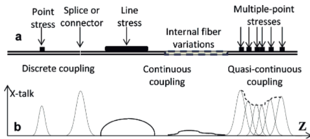
Fig. 1 Illustration of different types of polarization crosstalk. a) Different sources of polarization crosstalk. b) The resulting crosstalk peak profiles. Left: discrete polarization x-talk peaks induced by a point stress or a splice. Each such peak is a Gaussian curve with a shape determined by the coherence function of the light source. The spatial resolution is also determined by the width of the coherence function. Center: continuous polarization x-talk induced by a line stress and by internal fiber imperfections, respectively. Right: quasi-continuous x-talk induced by multiple densely packed stress points spaced on the order of or less than the resolution of the instrument.
