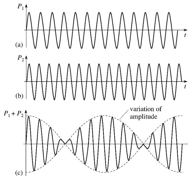
Figure 25 Interference pattern from two waves of differing frequency
