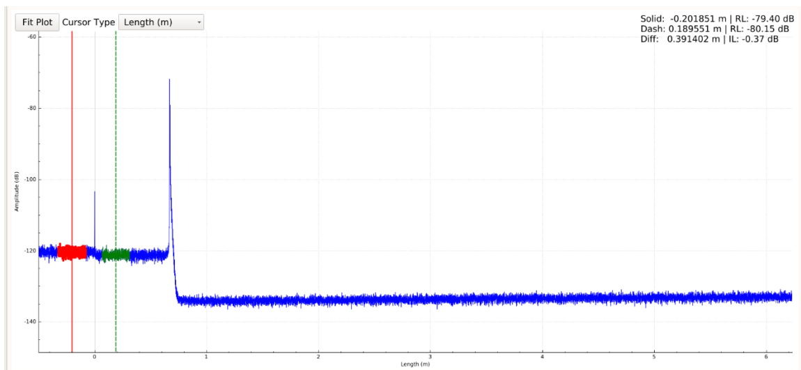
Figure 32 Insertion loss measurement shown across an APC fiber connector. (IL is shown in upper right corner)
