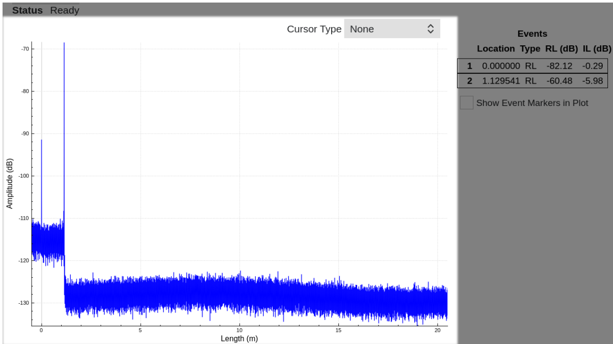
Figure 3 Delay Plot
