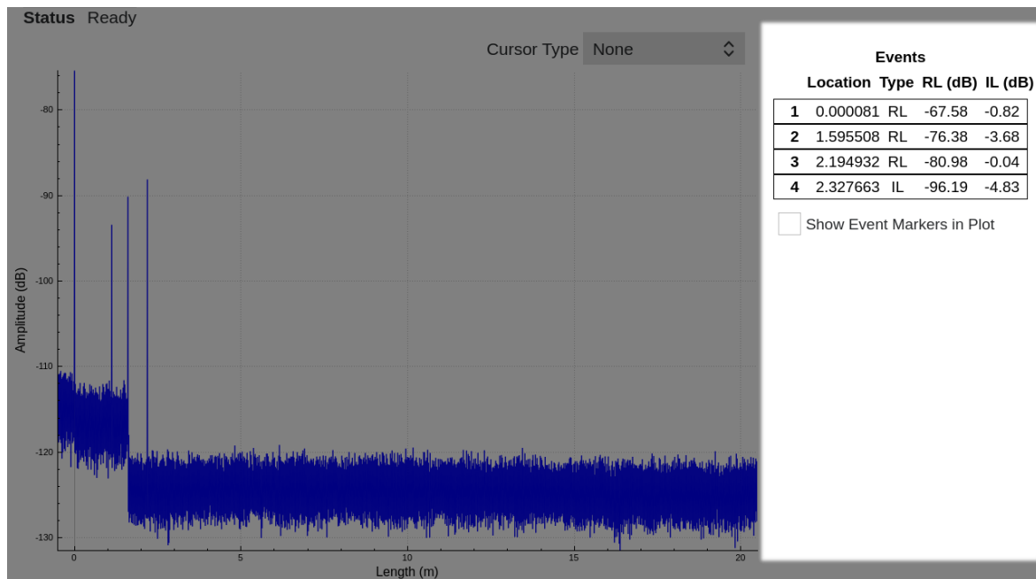
Figure 7 Event Table
