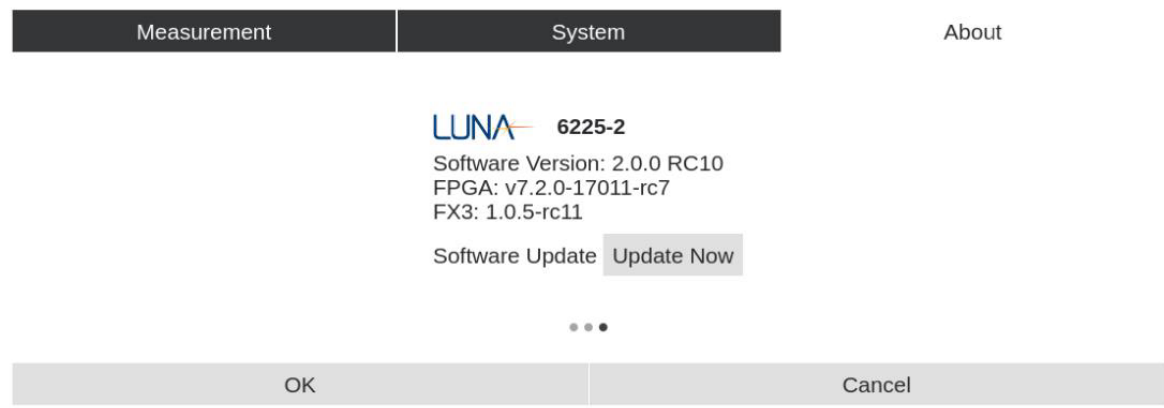
Figure 14 About Tab
