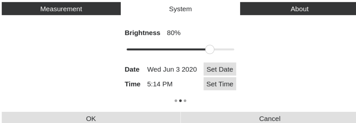
Figure 13 System tab
