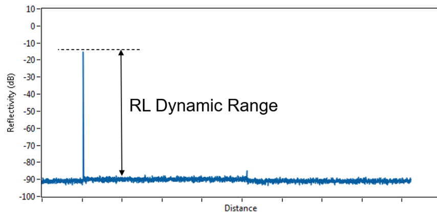
Figure 31 RL dynamic range limitation
