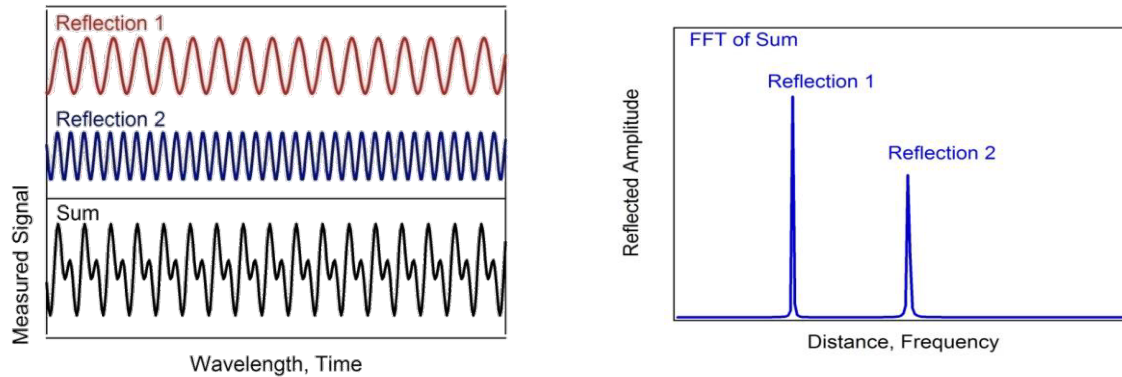
Figure 29 Resulting interference pattern from two reflectors at different locations
