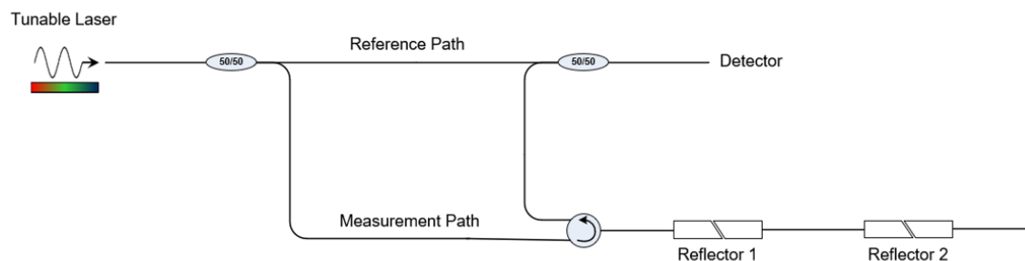
Figure 28 Basic OFDR Optical Network with two partial reflectors (connectors)
