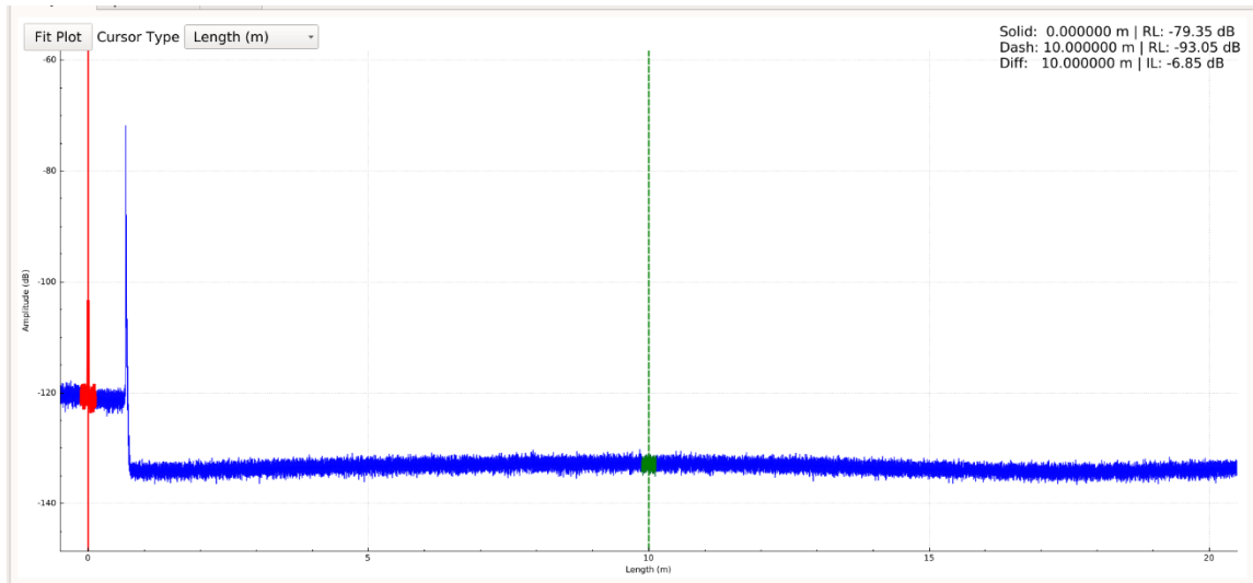
Figure 30 RL measurement using 0.25m RL integration width
