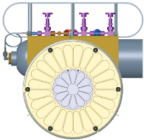
Bottom view of Model 107 ADR cryostat showing pulse-tube cooler and feedthrough flanges
