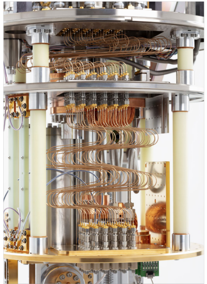
Close-up of HPD Model 106 ADR Cryostat
