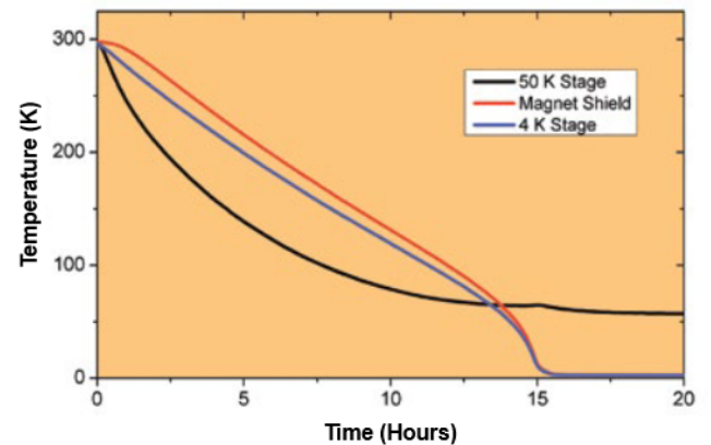
Typical Model 106 Cooldown Curve
