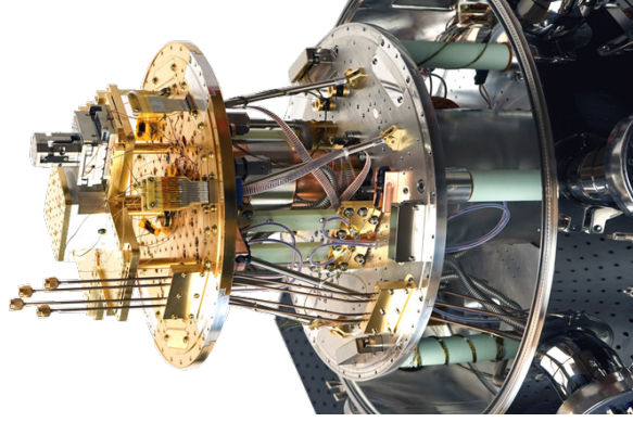
HPD Kilimanjaro 125 chip-scale semi-automated 4 K probe station with vibration isolation
