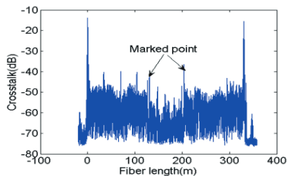
Figure 7 Identification of the locations of selected points on the fiber by inducing temporary stress on the fiber at these points.
