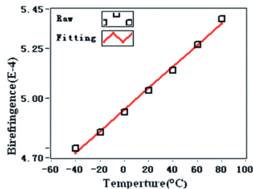
Figure 11 Linear fit to a plot of \Delta n vs. temperature for a PM fiber coil. The birefringence temperature variation coefficient 5.3E-7 can be obtained from the slope of the fitted line.
