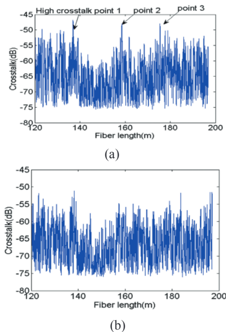
Figure 5 Polarization x-talk measurement results for layers 1-4 of a coil after initial winding (a) and after rewinding (b). Note that the high x-talk points observed during the initial winding are corrected by a more careful rewinding of the fiber.
