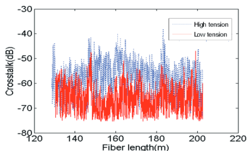
Figure 6 Polarization x-talk of layers 1-2 of a fiber coil wound at different tension levels. Solid line: low tension. Broken line: high tension
