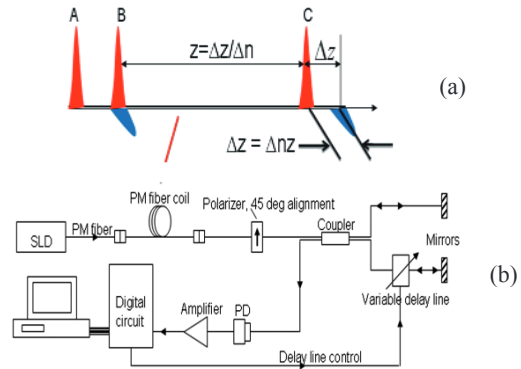
Figure 2 (a) Polarization crosstalk in a PM fiber. A single-polarization pulse is traveling in the fiber at point A. Crosstalk is induced by a stress at point B. The relative delay at output point C between the two pulses is \Delta Z . The location Z of x-talk point B can be obtained from a measurement of relative delay \Delta Z . (b) Structure of distributed polarization x-talk analyzer. A white light Michelson interferometer with a variable delay line is used to obtain the relative delay.
