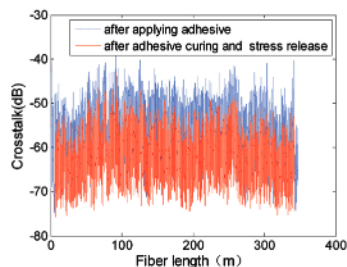
Figure 8 Polarization x-talk measurements of a PM coil after adhesive application and after adhesive curing and stress release. After adhesive curing and stress release (solid red line), the coil's average polarization x-talk decreases by 6dB relative to its level immediately after adhesive application (dashed blue line).
