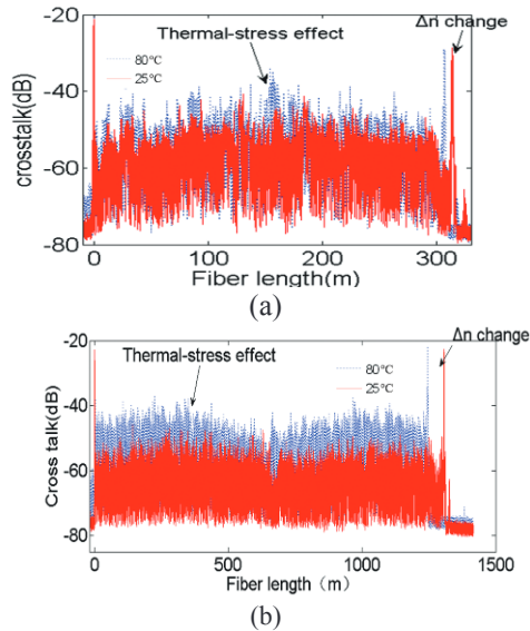
Figure 10 Changes in polarization x-talk of 315 m and 1300 m PMF coils due to thermal-stress effects. (a) 315 m coil (b) 1300 m coil.
