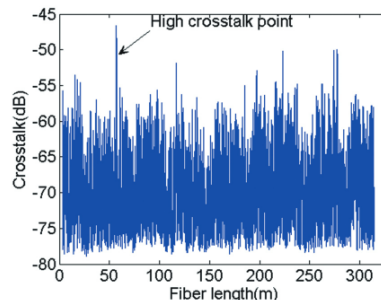
Figure 9 Polarization x-talk profile of a 311 m PMF coil. The overall polarization x-talk is relatively low for this coil; however, some high x-talk points can still be observed.
