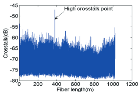
Figure 3 Polarization x-talk measurement of 1000 m of raw fiber. High x-talk (-47 dB) is observed at 381 m.
