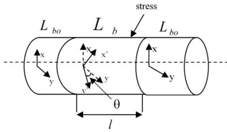
Figure 1 Model of the mechanism of polarization x-talk in PM fiber. The stress on the center section causes a relative rotation of the birefringence axes and hence the polarization x-talk.
