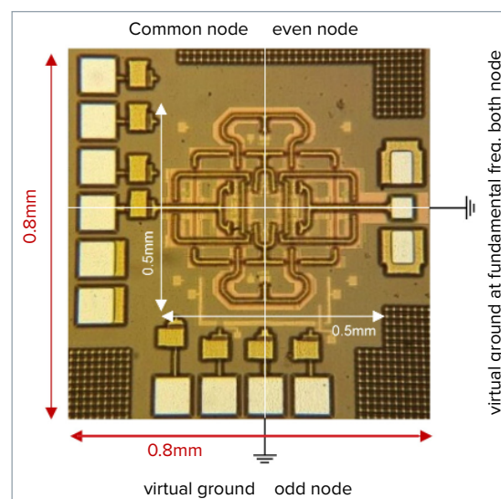
Figure 1: A BiCMOS process with a 135 nm feature size was used to fabricate the VCO. The pads on the left and bottom were wirebonded to a mounting board to provide power supplies and control voltages. The two pads on the right were the oscillator output and the targets of the Infinity Probes.
