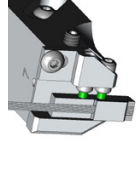
Vertical array holder, 4° to 20°, arrays up to 4.2 mm wide
