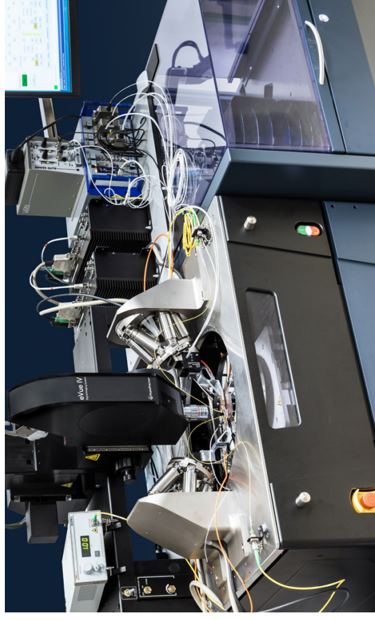
Silicon Photonics Measurement Assistant on FormFactor's 200 mm probe station SUMMIT200
