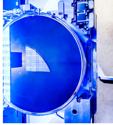
Pull-out chuck with OptoVue Pro 200 in the auxiliary chuck positions - SUMMIT200
