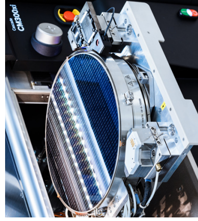
Pull-out chuck with OptoVue Pro in the auxiliary chuck position - CM300xi
