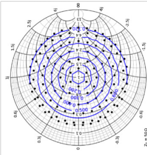
Figure 9: Tuning range at 28 GHz with RF TopHat. \Gamma_{max} = 0.74 , \Gamma_{mic\_280log} = 0.7
