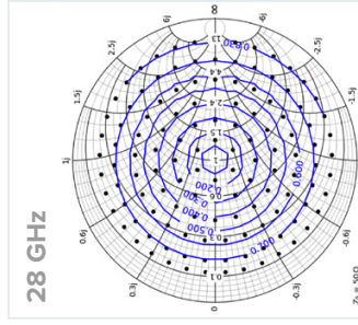
Figure 4: Tuning range at 28 GHz: \Gamma_{max} = 0.84 , \Gamma_{max\_360deg} = 0.79
