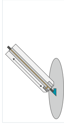
Figure 3: Shortened measurement path: FormFactor's Infinity probe is directly connected to the DELTA tuner from Focus Microwaves.
