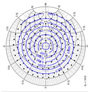
Figure 8: Tuning range at 28 GHz without RF TopHat. \Gamma_{max} = 0.84 , \Gamma_{mic\_280log} = 0.79
