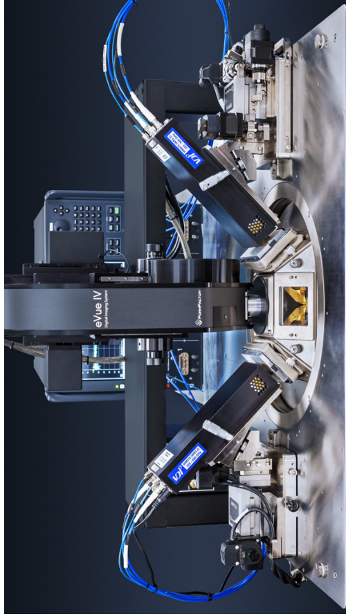
mm-Wave probing on a SUMMIT200. The solution is also available for all other probe systems from FormFactor.
