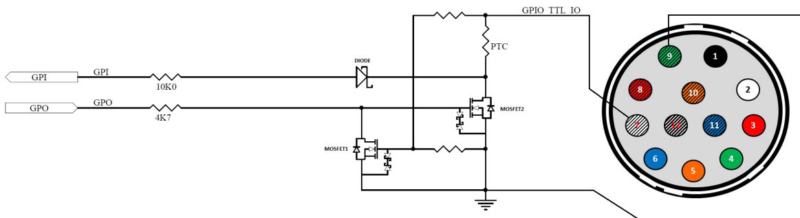
Input/Output circuit
