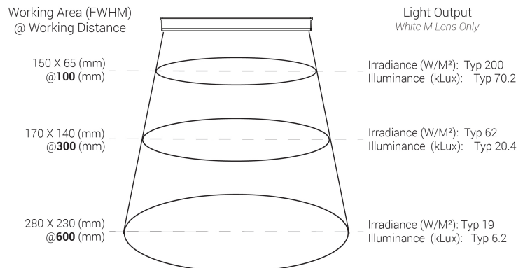
Optical Cone
