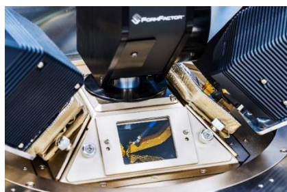
FormFactor T-Wave Dual band probe with integrated diplexer
